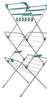
Extendable 3 tier airer Folded: w 440 x h 510 x d 90mm Fully extended: w 720 x h 1040 x d 380mm
